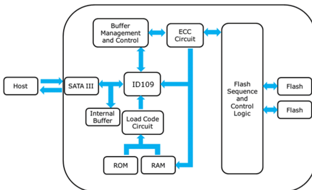
Figure 2: Innodisk M.2 (S42) 3ME3 Block Diagram
